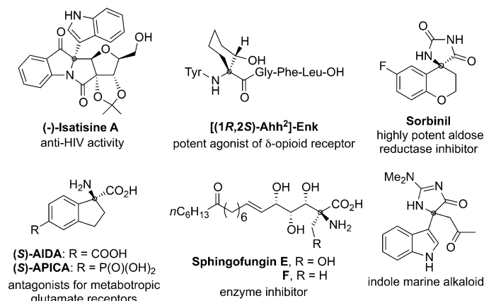
Scheme 1. Selected medicinal and natural molecules containing \alpha,\alpha -disubstituted \alpha -amino acids and their derivatives.
